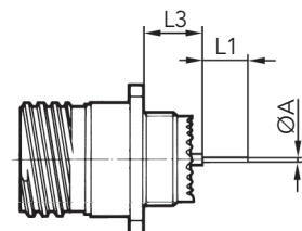
Receptacle type 00
